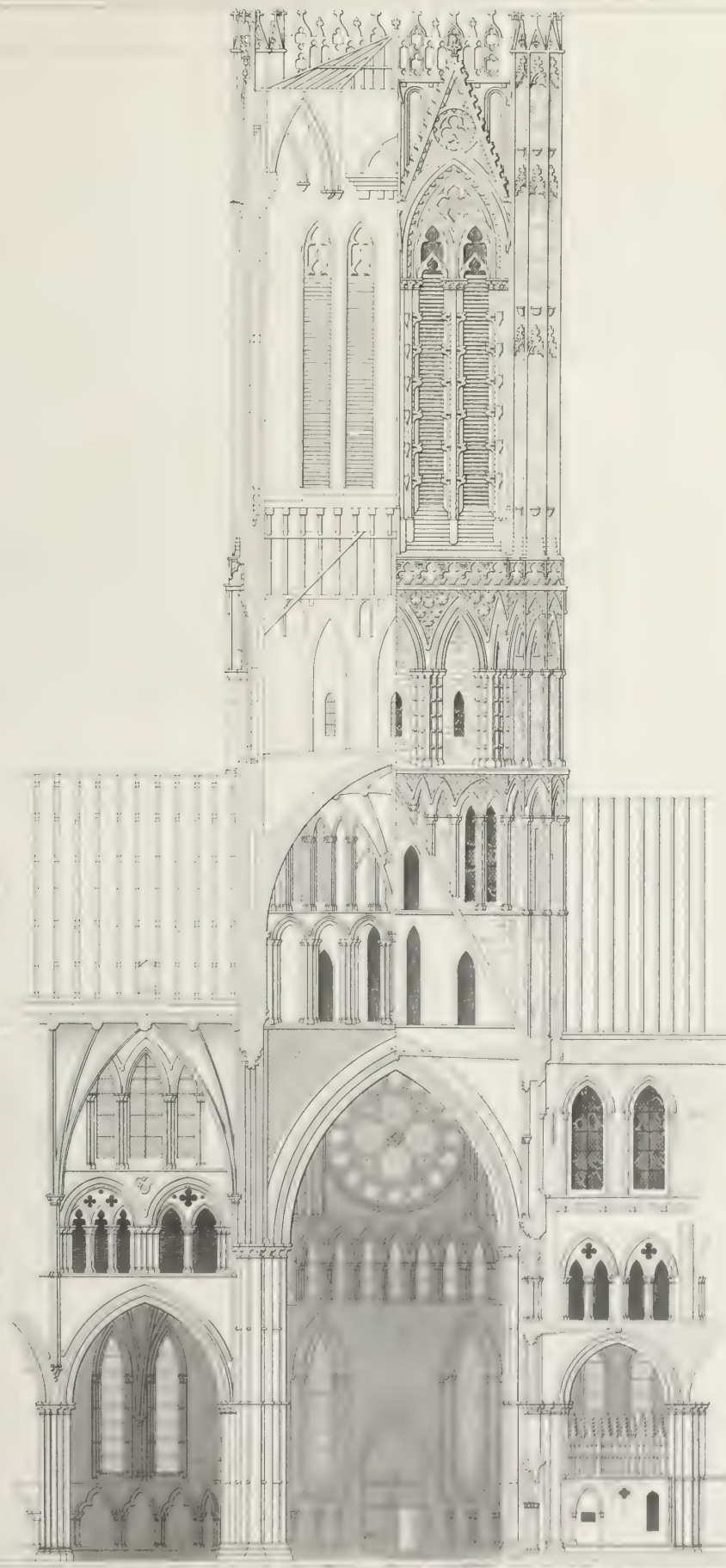
SECTION OF THE CATHEDRAL OF SALISBURY, SHOWING THE INTERIOR OF THE CHANCEL AND THE TOWER OF THE SPIRE.
